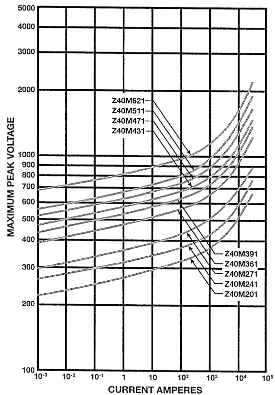
Z40M Series Voltage VS Current Characteristics
