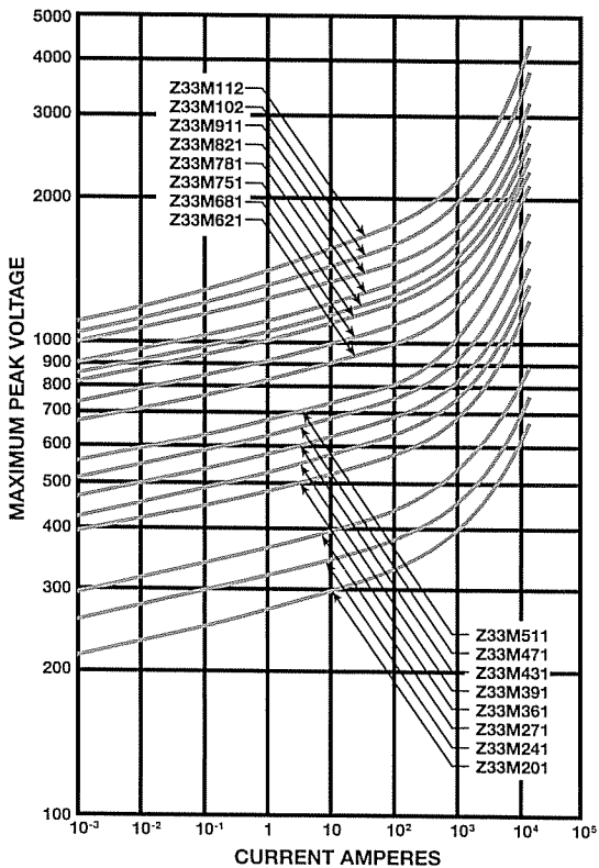
Z33M Series Voltage VS Current Characteristics
