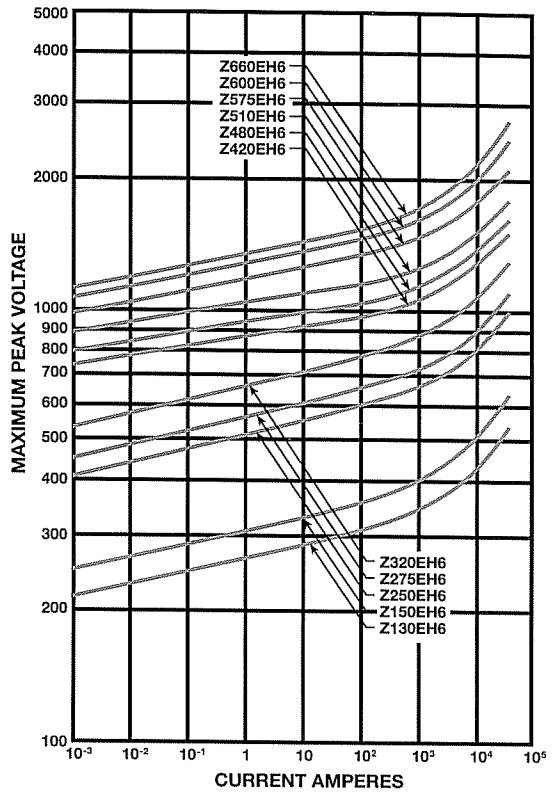
EH Series Voltage VS Current Characteristics
