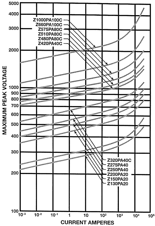
PA Series Voltage VS Current Characteristics
